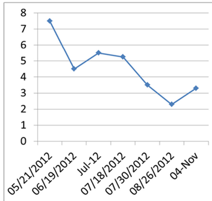
Secchi Depth in meters
